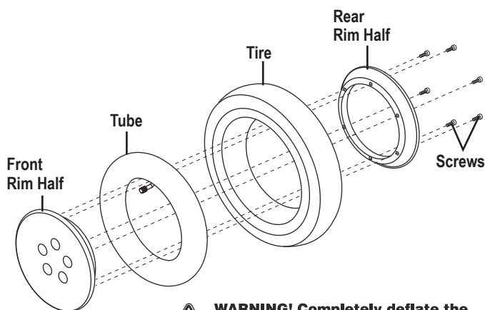
Figure 14. Drive Wheel Disassembled
