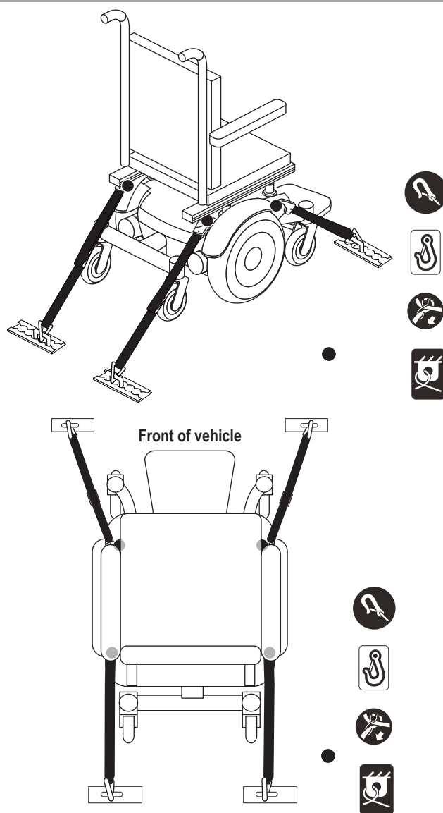
Figure 7. Unoccupied Transit System Securement Points
